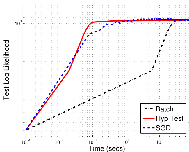
Figure 3: Test log-likelihood as a function of time for logistic regression on the MNIST dataset.
