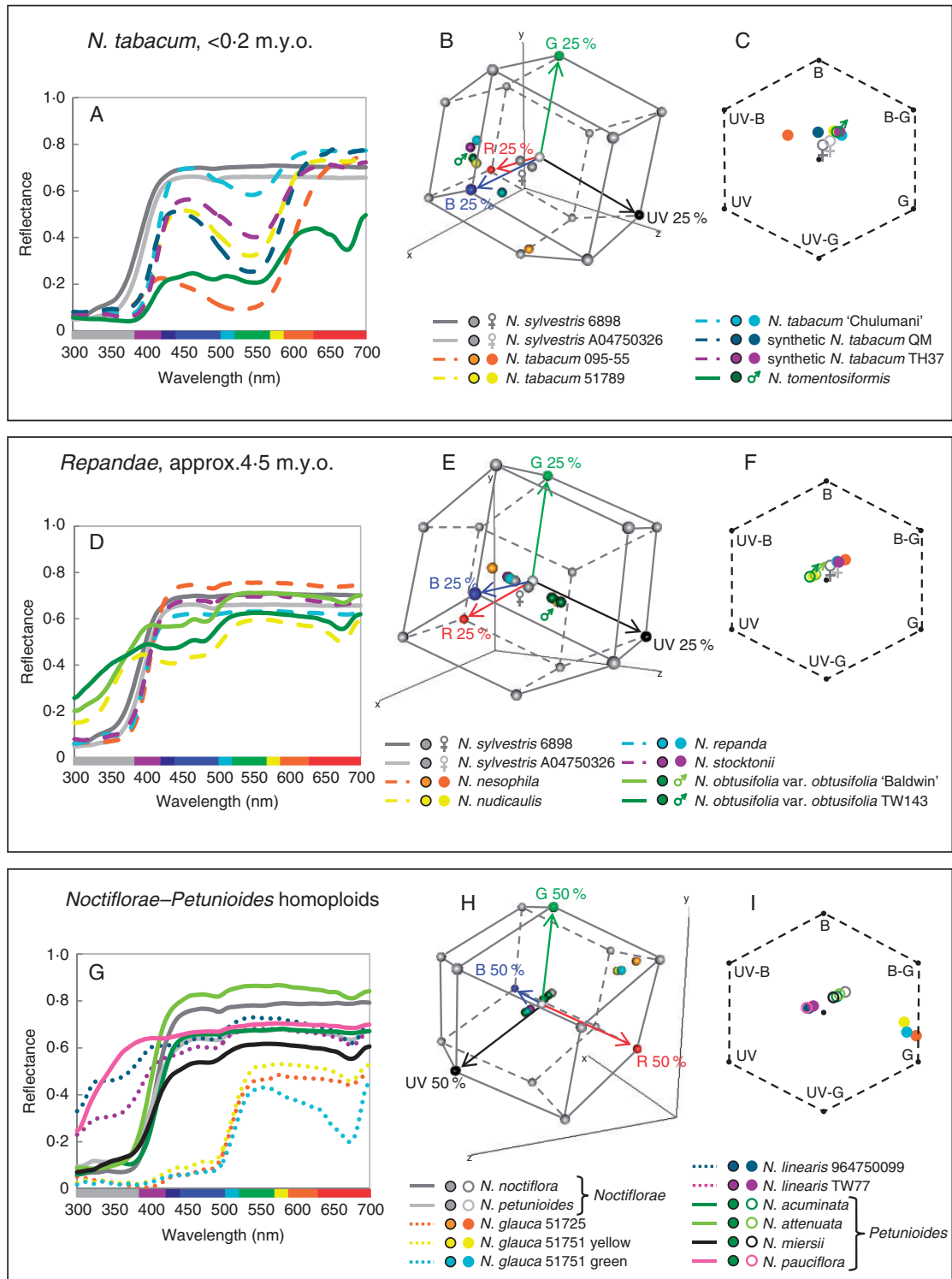
FIG. 5. (A, D, G) Reflectance spectra for polyploid and homoploid sections and their progenitors: (A) N. tabacum ; (D) section Rebandae ; and (G) Noctiflorae–Petunioides homoploid hybrids. Solid lines are used for diploid taxa, dashed lines for polyploid taxa and dotted lines for homoploid hybrid taxa. (B, E, H) Hummingbird colour space for polyploid and homoploid sections and their progenitors: (B) N. tabacum ; (E) section Rebandae ; and (H) Noctiflorae–Petunioides homoploid hybrids. The vertices of the hummingbird colour space represent 25% (B, E) or 50% (H) excitation of the photoreceptors; single photoreceptor type vertices (red, green, blue and UV) are coloured red, green, blue and black, respectively, and all other vertices are grey. Red, green, blue and black arrows represent the vectors of these photoreceptors from the origin of the hummingbird colour space. (C, F, I) Bee colour spaces for polyploid or homoploid sections and their progenitors: (C) N. tabacum ; (F) section Rebandae ; and (I) Noctiflorae–Petunioides homoploid hybrids. Hexagons have been scaled so that vertices represent 40% excitation of photoreceptors. UV, ultraviolet; UV-B, UV-blue; B, blue; B-G, blue-green; G, green; UV-G, UV-green. For information regarding how to interpret colour hexagons, see Supplementary Data Fig. S1 . Female (♀) and male (♂) symbols mark maternal and paternal progenitors, respectively, in the hummingbird and bee colour spaces.
