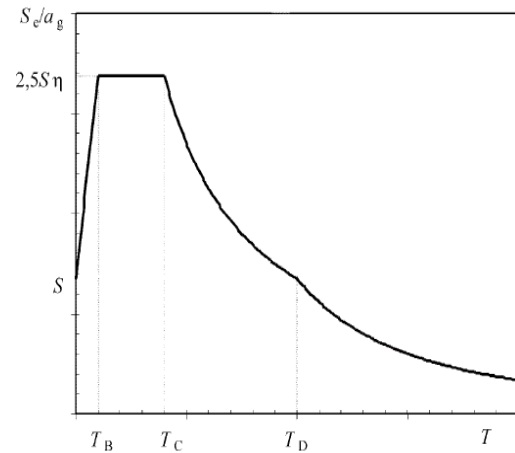
Figure 1: General shape of Response Spectra
